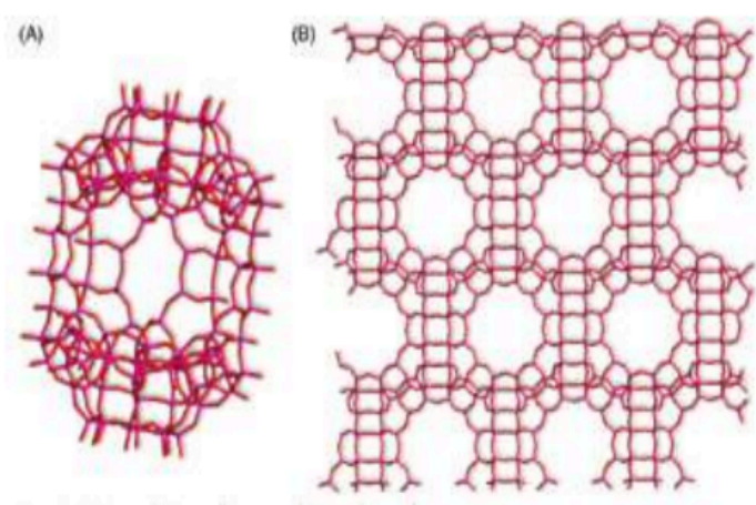
Figure 8. SBE framework (A) unit cell/supercage and (B) view along
