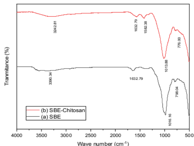
Figure 2. (a) Infrared spectrum SBE and (b) SBE Chitosan composite
