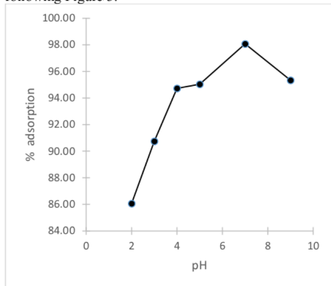
Figure 3. Effect of pH on % adsorption Fe(III)
