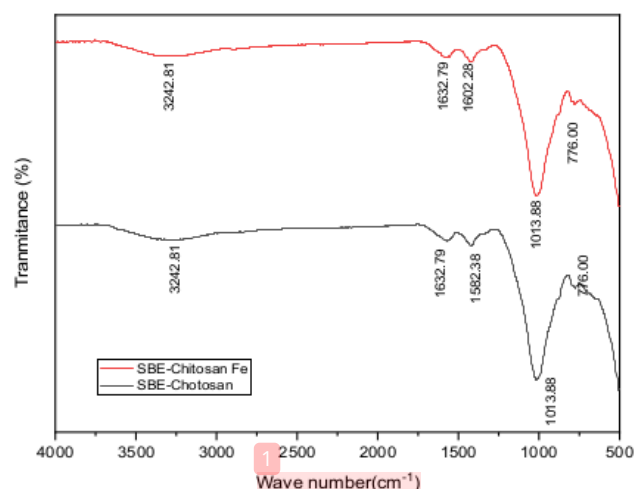
Figure 9. FTIR Spectrum of the SBE-Chitosan and the SBE-chitosan composite after adsorption Fe(III)
