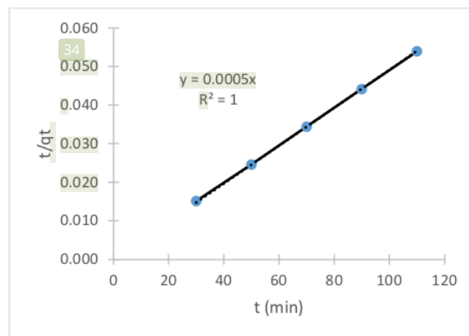
Figure 5. Pseudo-second-order kinetics of the uptake adsorption Fe(III) on SBE chitosan composite
