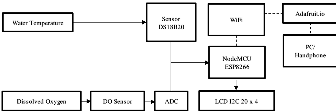
Figure 1. Proposed system block diagram
