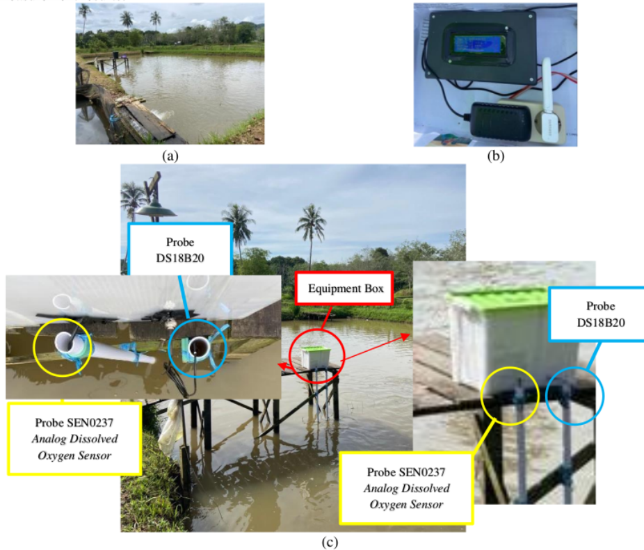
Figure 3. (a) Location of catfish ponds where data is collected, and (b) Measurement and IoT system processing equipment, and (c) IoT based monitoring system for temperature and dissolved oxygen levels in catfish farming ponds
