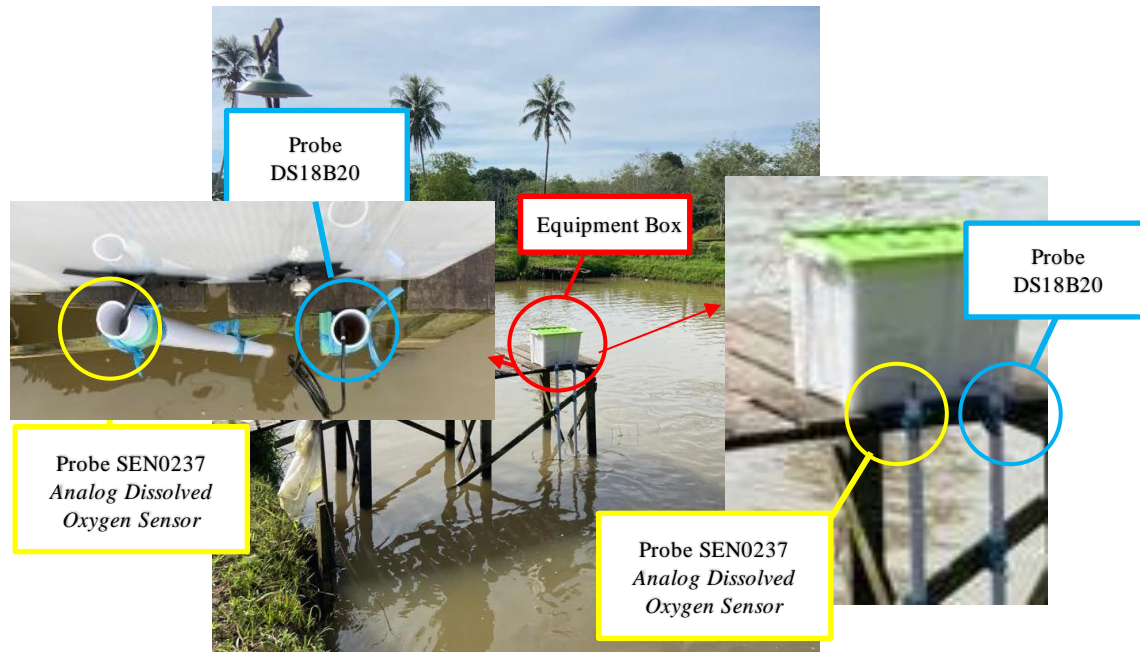
Figure 6. (a) Location of catfish ponds where data is collected, and (b) Measurement and IoT system processing equipment, and (c) IoT based monitoring system for temperature and dissolved oxygen levels in catfish farming ponds
