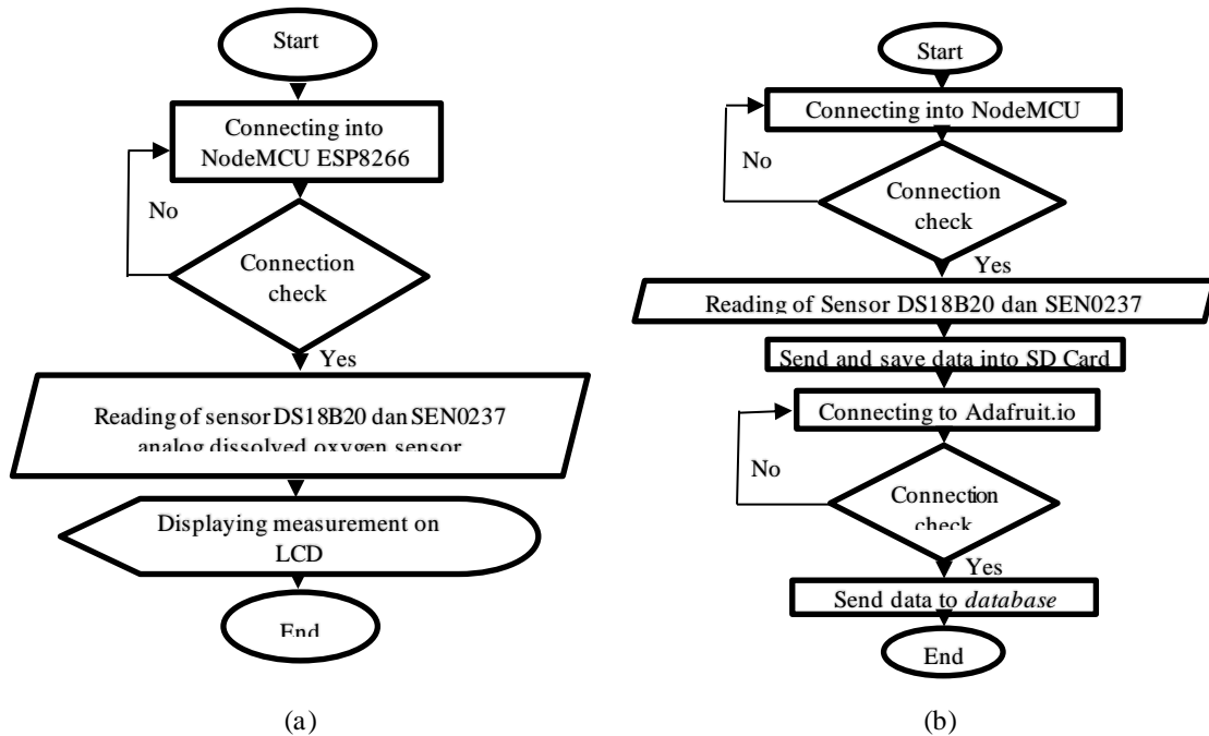
Figure 2. Flowchart of (a) NodeMCU ESP8266 with sensors and LCD, and (b) NodeMCU ESP8266 with IoT
