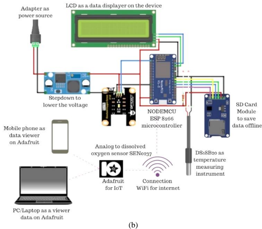
Figure 1. Proposed system of (a) block diagram and (b) circuit design
