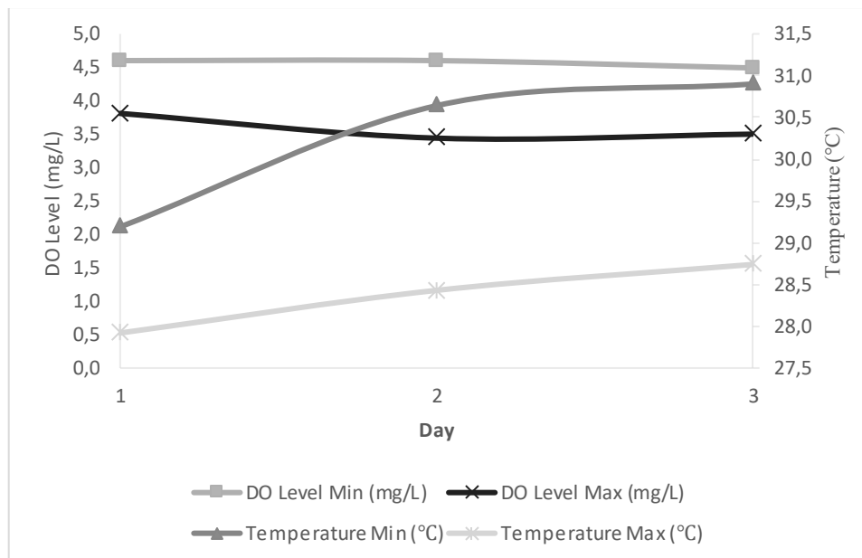
Figure 8. The maximum and minimum values of DO Level and temperature of 3 days of measurement
