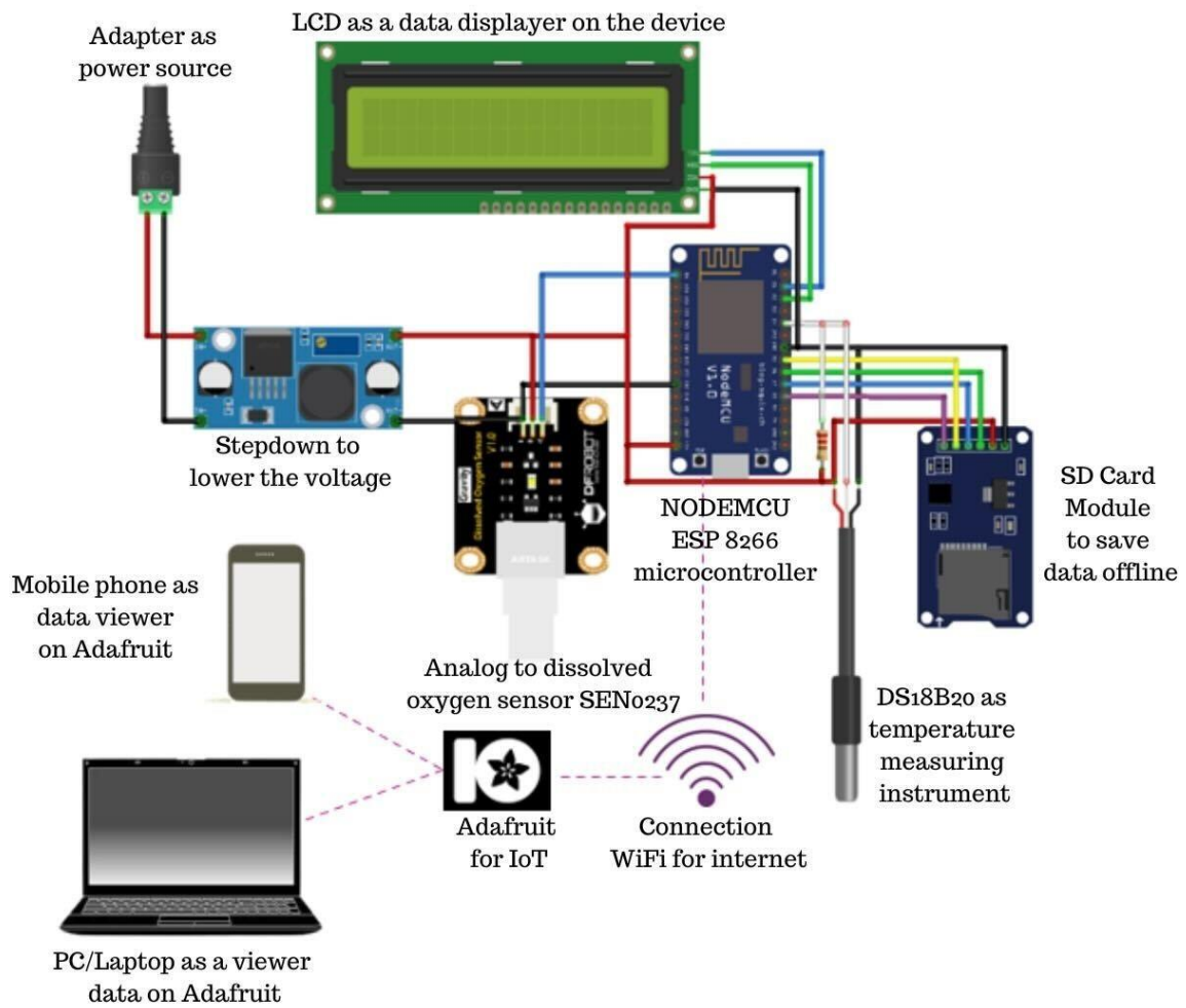
Figure 1. Proposed system, (a) Block diagram, (b) Circuit design
