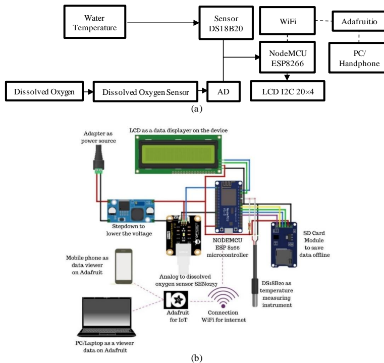
Figure 1. Proposed system of (a) block diagram and (b) circuit design
