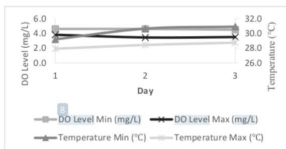
Figure 8. The maximum and minimum values of DO Level and temperature of 3 days of measurement
