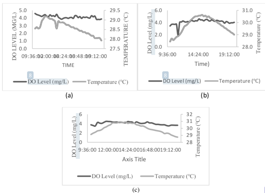
Figure 7. Data collection of DO Level (black line) and Temperature (gray line) for three days, (a) First day data collection, (b) Second day data collection, and (c) (a) Third day data collection, 23
