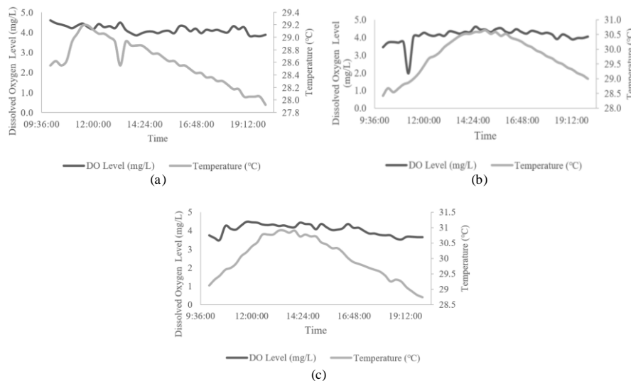
Figure 7. Data collection of dissolved oxygen level (black line) and temperature (gray line) for three days (a) first day, (b) second day, and (c) third day data collection
