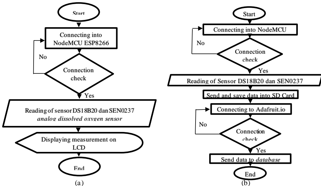
Figure 2. Flowchart of (a) NodeMCU ESP8266 with sensors and LCD, and (b) NodeMCU ESP8266 with IoT
