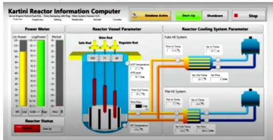
Figure 1. RL Kartini in the reactor power calibration practicum
