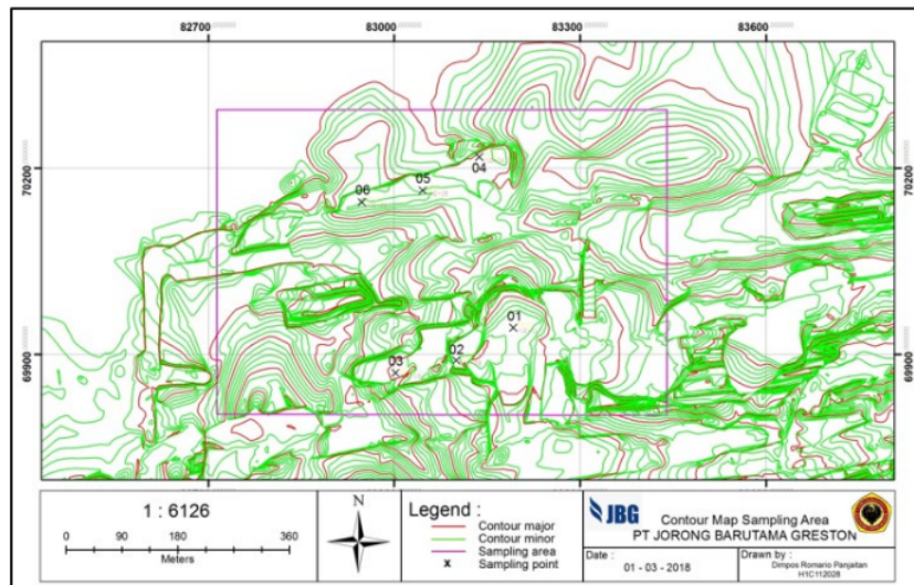
Gambar-2. Contour Map Sampling Area
