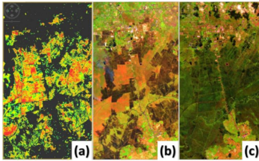
Figure 4. (a) Burned area from RBR, (b) Burned area on postfires imagery, and (c) Regrowth imagery
