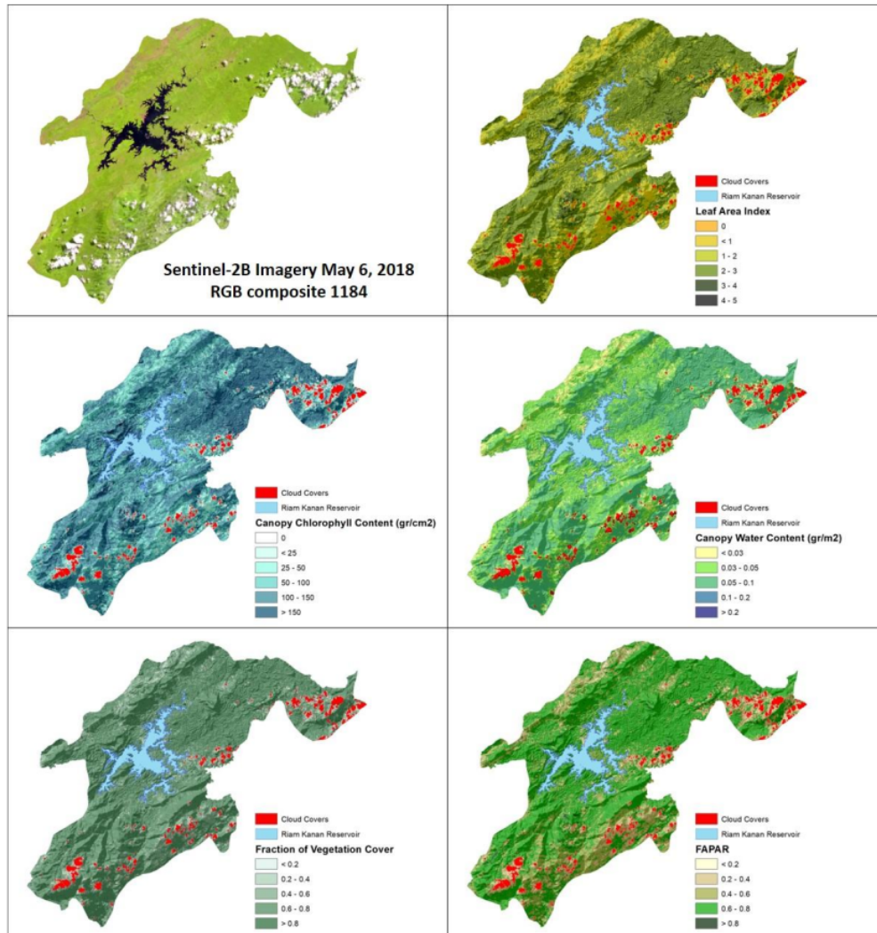
Figure 4. Sentinel-2B imagery and biophysical parameters
