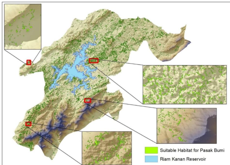
Figure 5. Habitat suitability of pasak bumi
