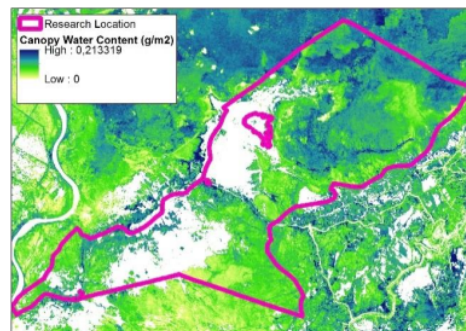
Fig. 9. CWC imagery.
