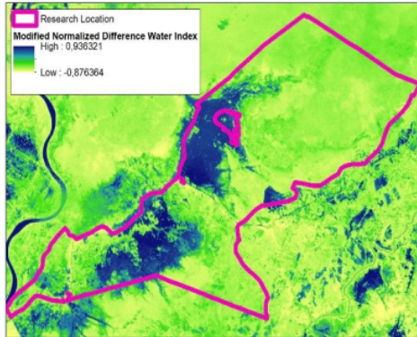
Fig. 10. MNDWI imagery.
