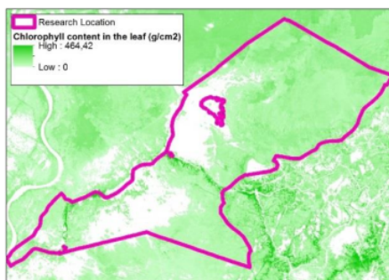
Fig. 7. CCC imagery.
