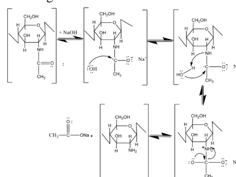
Figure 2. Chitosan synthesis reaction mechanism.[9]
