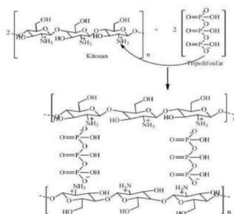
Figure 7. Chitosan Reaction Mechanism with NaTPP.15
