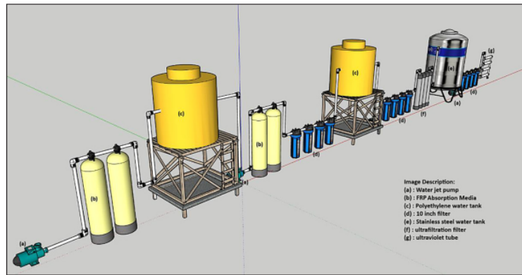
Figure 5. Single flow ultrafiltration
