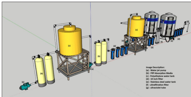
Figure 4. Double flow ultrafiltration
