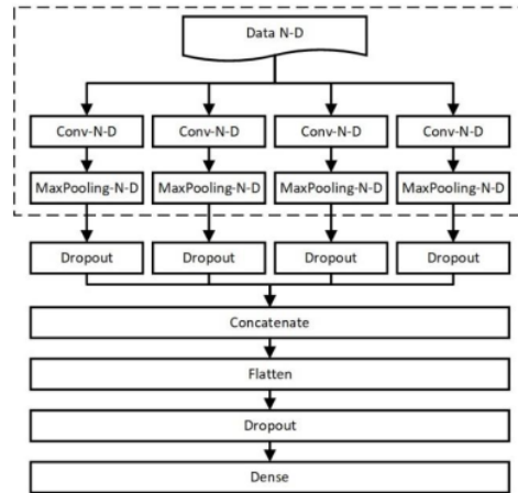
Figure 5. N-D CNN Architecture.
