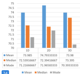
Figure 10. Comparison of average accuracy based on word padding technique in sentences.
