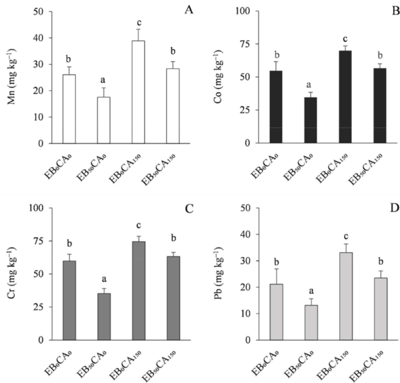
Figure 4. Effect of empty fruit bunch of 71 palm (EB) and coal fly ash (CA) applications on Mn (A), Co (B), Cr (C), and Pb (D) in plant tissue. The lines above bars represent standard deviation of the mean (n=5). Similar letters above the lines indicate the effect of the treatments is not significantly different based on the least significant difference (LSD) test at p<0.05.
