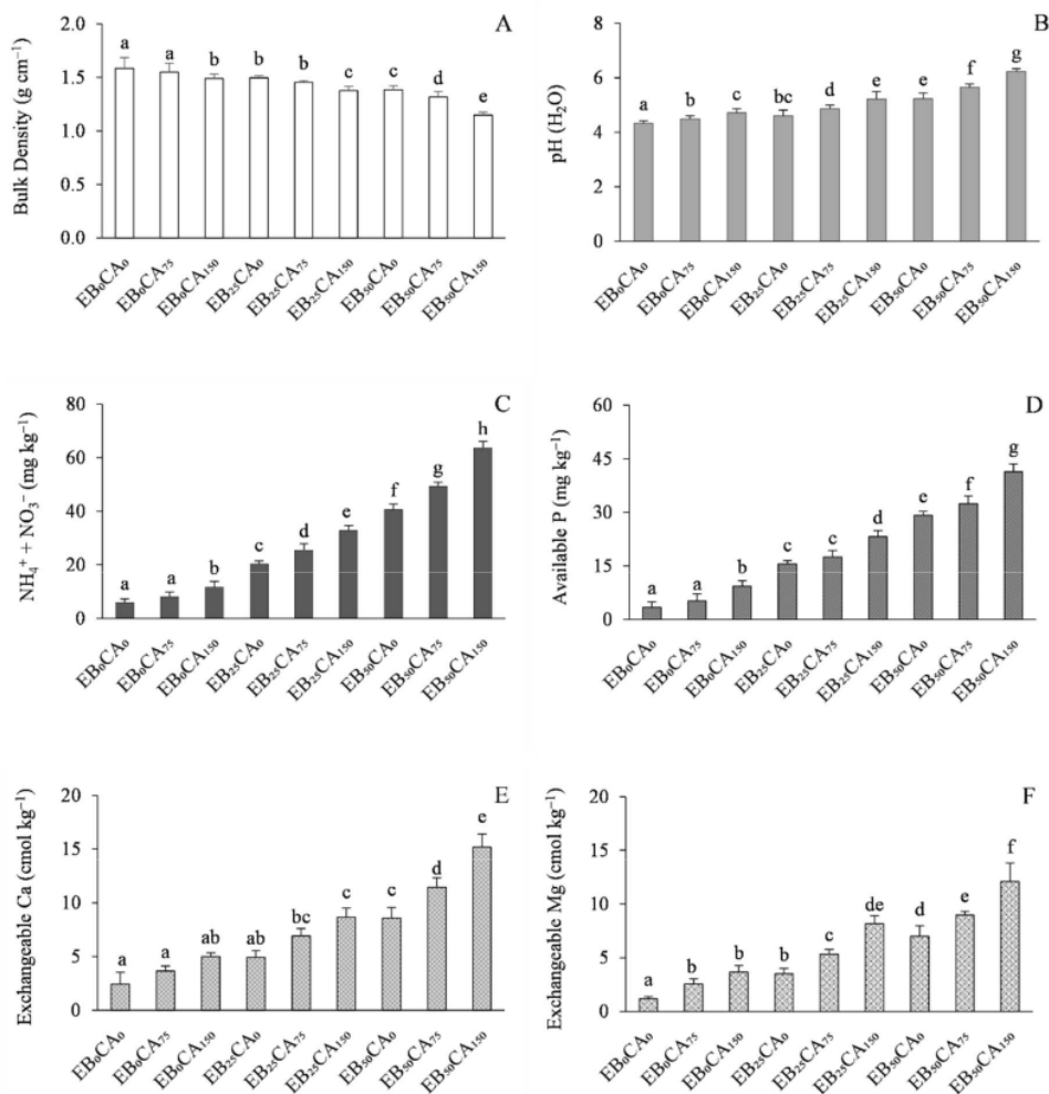
Figure 2. Changes in bulk density (A), pH (B), mineral N ( NH_4^+ and NO_3^- ) (C), available P (D), exchangeable Ca (E), and exchangeable Mg (F) as influenced by different amounts of empty fruit bunch of oil palm (EB) and coal fly ash (CA) applications. The lines above bars represent the standard deviation of the mean ( n=3 ). Similar letters above the lines indicate the effect of the treatments is not significantly different based on the least significant difference (LSD) test at p<0.05 .
