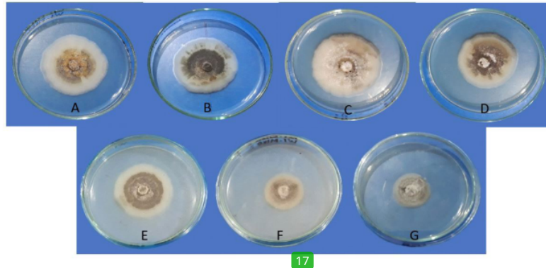
25 2. Visual comparison of the growth of C. capsici in the addition of liquid smoke with a concentration of (A) 0.00% (B) 0.085% (C) 0.17% (D) 0.34% (E) 0.68% (F) 1.36% (G) 1.75% of the 7th day of incubation.
