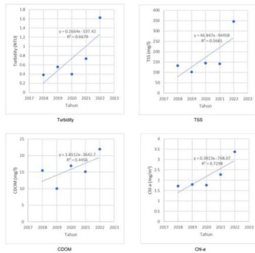
Fig 8:- Water quality trendline
