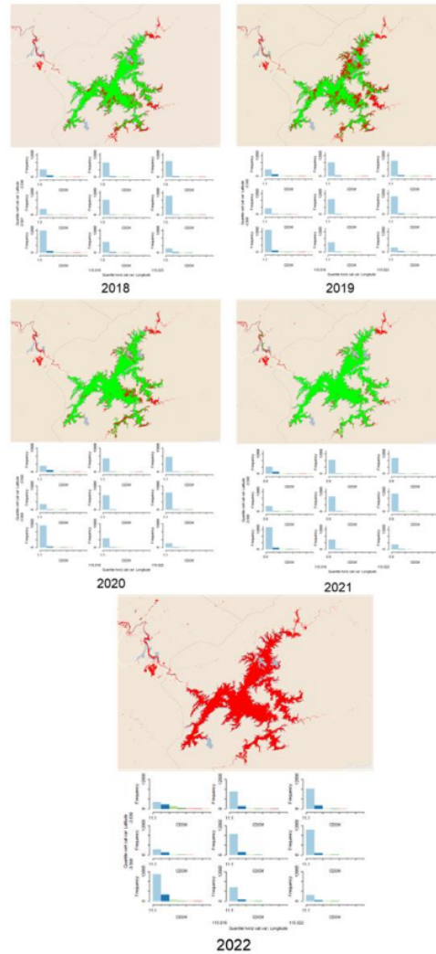
Fig 7:- Distribution of CDOM in the lake
