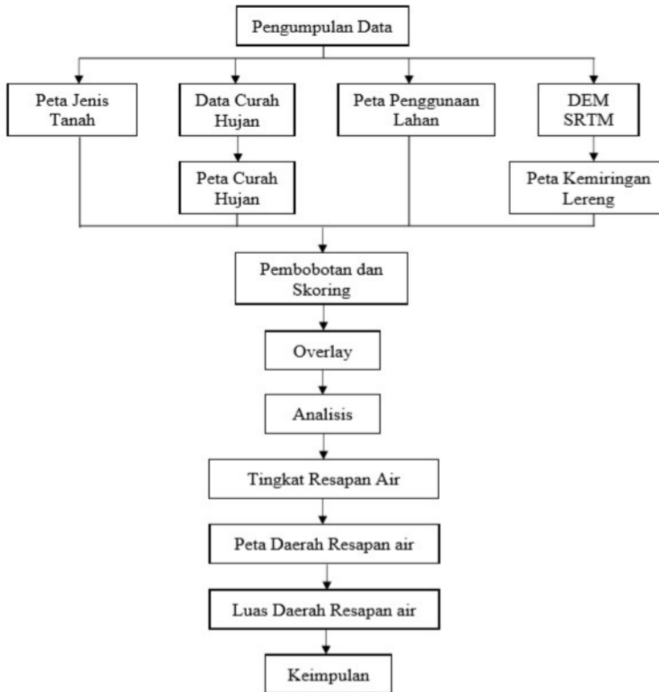
Gambar 2 Diagram Penelitian
