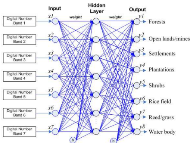
Fig. 3. Architecture of ANN back propagation
