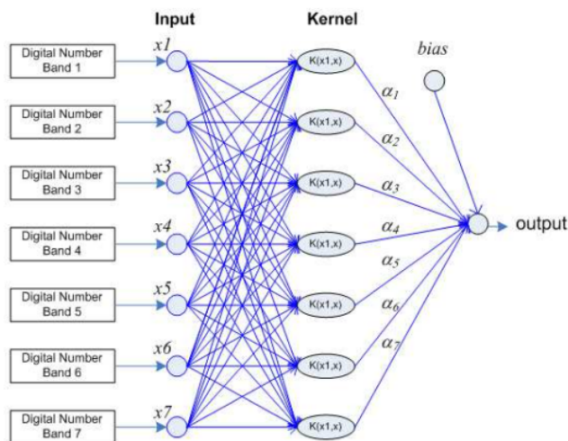
Fig. 2. Architecture of SVM
