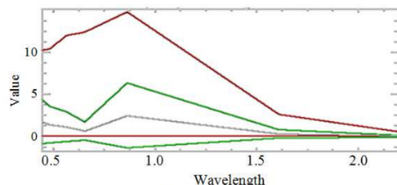
Fig. 4. Graph of min, max and mean values on each band 1-7 before radiometric correction (Source: Data processing, 2015)
