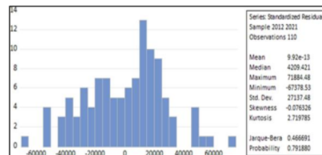
Fig. 1. Normality test result.
