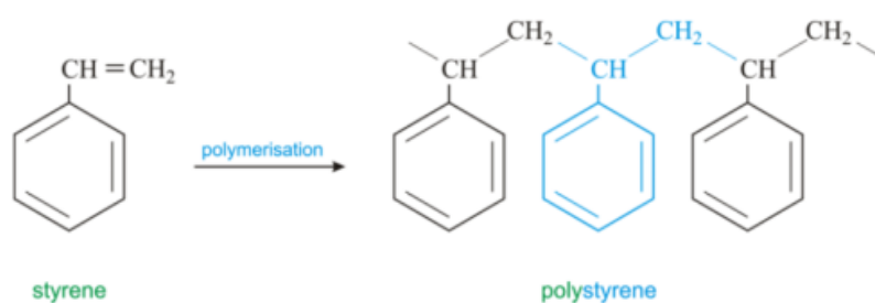
Fig. 5. Process of Polystyrene made (source: https://europilas.com.vn/en-US/blog-1/everything-you-need-to-know-about-polystyrene )
