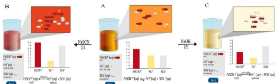
Figure 3. Simulation Result of The Effect of Concentration on Ion \text{FeSCN}^{2+} Equilibrium
