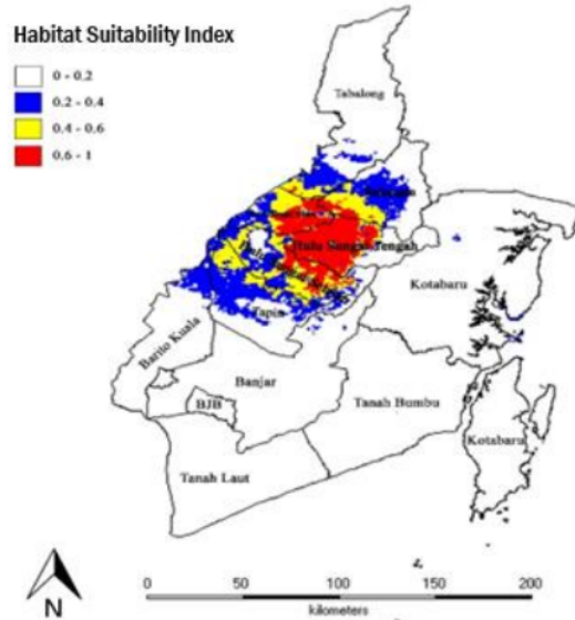
Figure 2. Map of suitable habitat for Mangifera rufocostata
