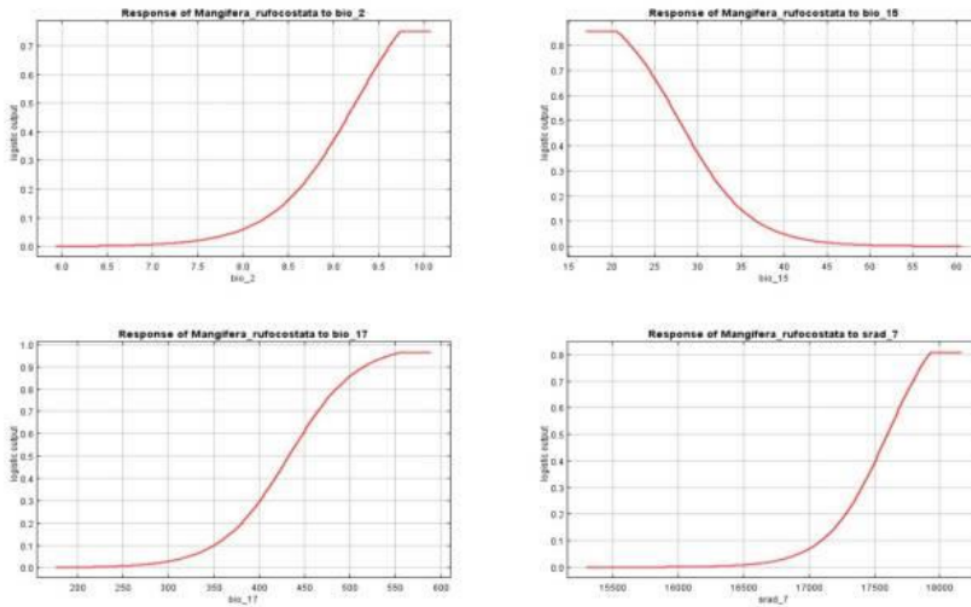
Figure 4. Response of environmental variables (bio_2=mean temperature, bio_15= precipitation seasonality, bio_17= precipitation, srad_7=solar radiation) to the presence of Mangifera rufocostata
