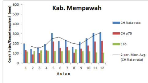
Figure 5. Monsoonal and Equatorial Rainfall Patterns and Water Balance of the Study Area
