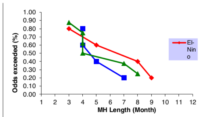
Figure 11. MH long prediction based on SOI phase
