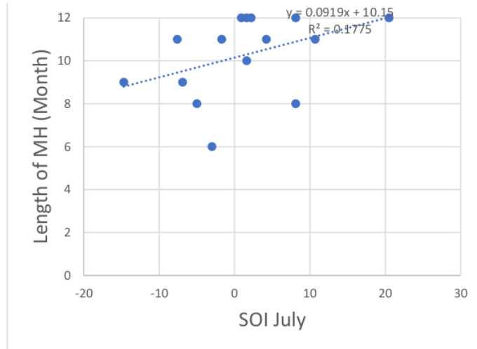
Figure 9. Connection between SOI July with Season Length Rain (Moonth) in Sambas/ Bengkayang area
