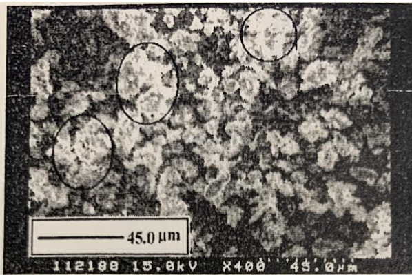
b. Soil with 0.2% cement content
