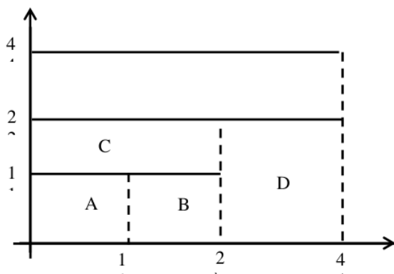
Figure 9- Curva Species Area (CSA) Plot Note. A: Plot 1 m x 1m; B: Plot 1 m x 2 m; C: Plot 2 m x 2 m; D: Plot 2 m x 4 m and so on until there are no more additional individuals
