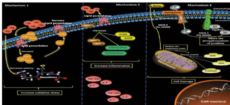
Figure 4. Mechanism of Mercury Induced Oxidative Stress 12
