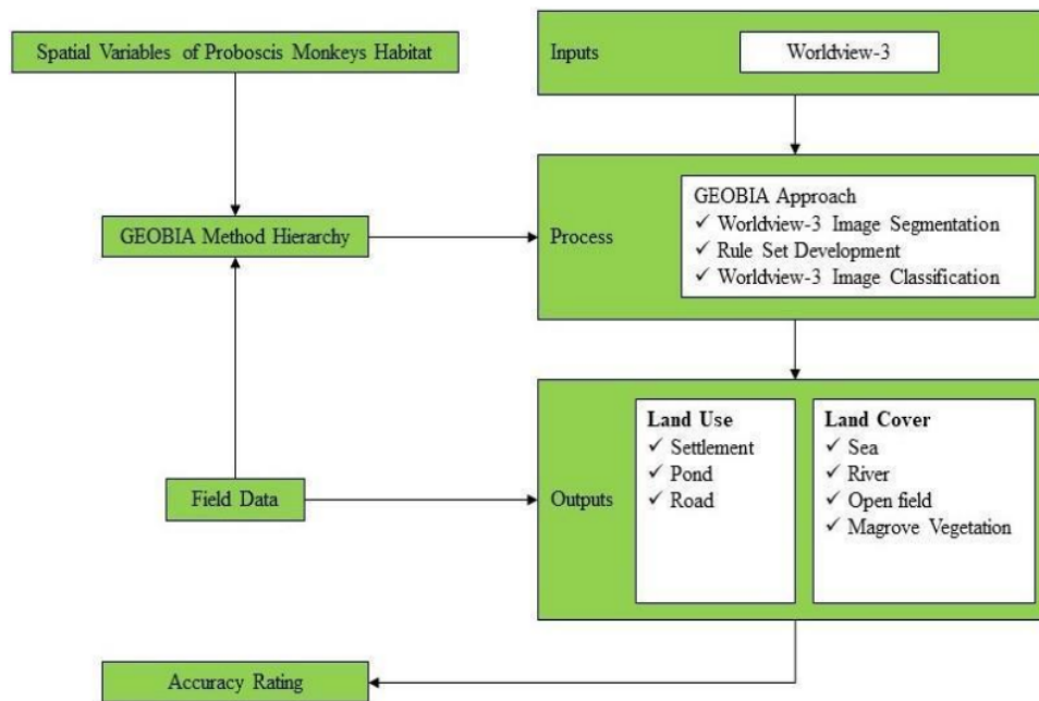
6 Figure 2 Schematic of land use and land cover classification process using GEOBIA analysis
