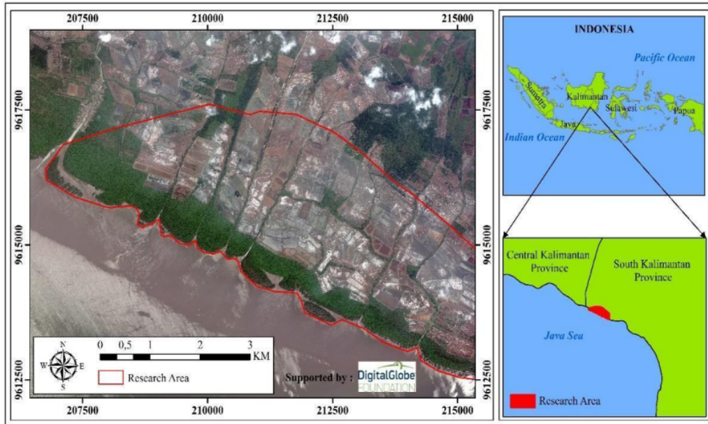
Figure 1 Research location of Kuala Lupak Wildlife Reserve
