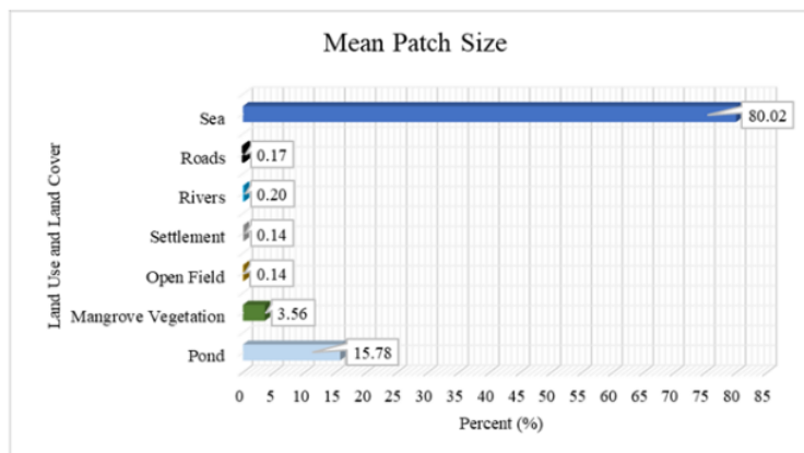
Figure 8 Graph of the mean patch size for each class in the Kuala Lupak Wildlife Reserve
