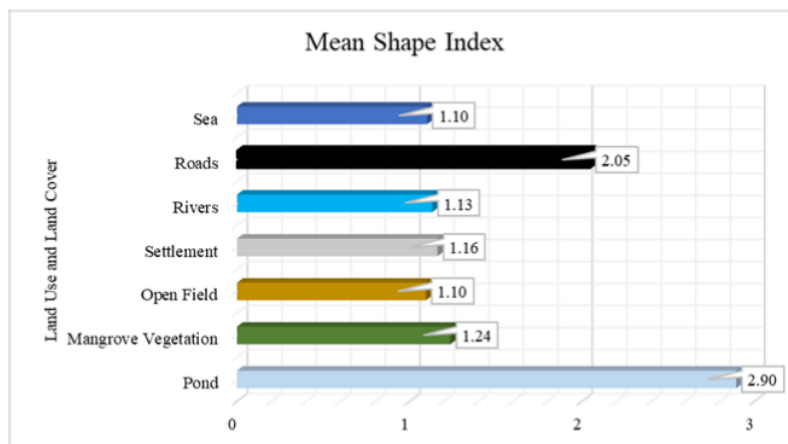
Figure 9 Graph of mean shape index for each land cover class in Kuala Lupak Wildlife Refuge
