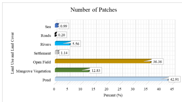
Figure 5 Graph of the number of patches for each class at the Kuala Lupak Wildlife Reserve
