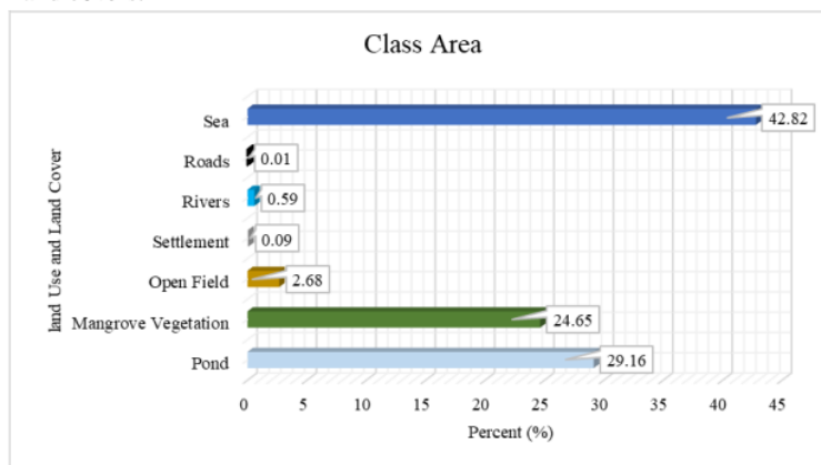
Figure 4 Compilers of the landscape of the Kuala Lupak Wildlife Reserve based on class area analysis
