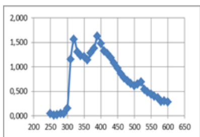
Figure 2. Wavelength Graph of Binjai Leaf Extract
