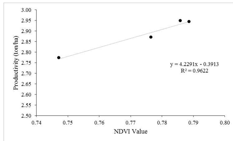
Figure 10. NDVI Coefficient of Determination and Productivity
