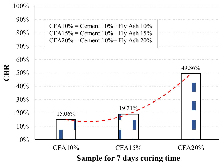
Figure 2. CBR test result
