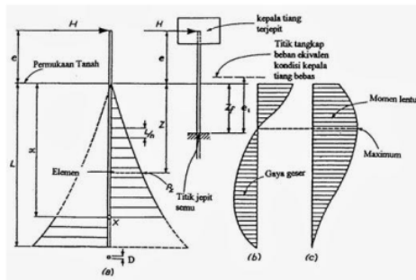
Figure 1 Brinch Hansen Method (1961)
