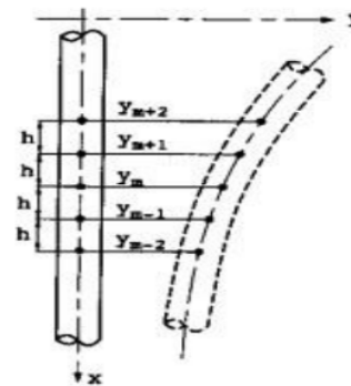
Figure 3 Deflection on the pile per depth (Prakash dan Sharma, 1990)
