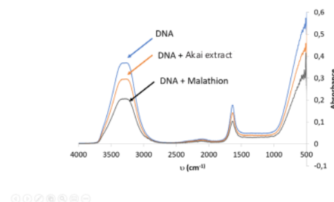
Figure 2: Spectra of FTIR DNA
