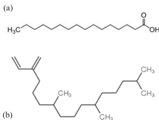
Figure 1: Hexadecanoic Acid (a) dan Neophytadiene (b)
