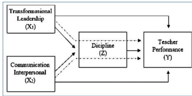
Fig-1: Path Model
