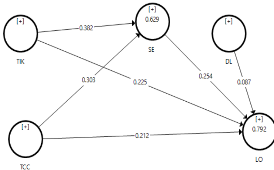
Figure 2 Measurement Model
