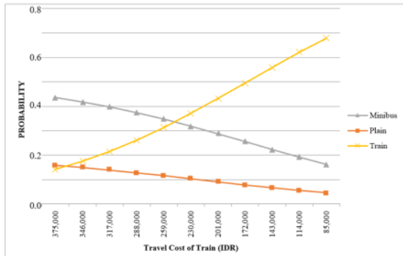
Figure 1. The graph of the sensitivity of the travel cost against the probability of mode choice modes
