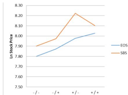
Figure 1. Interaction Pattern
