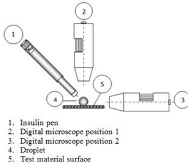
Figure 1. Experimental tool settings for droplet contact angle measurements
