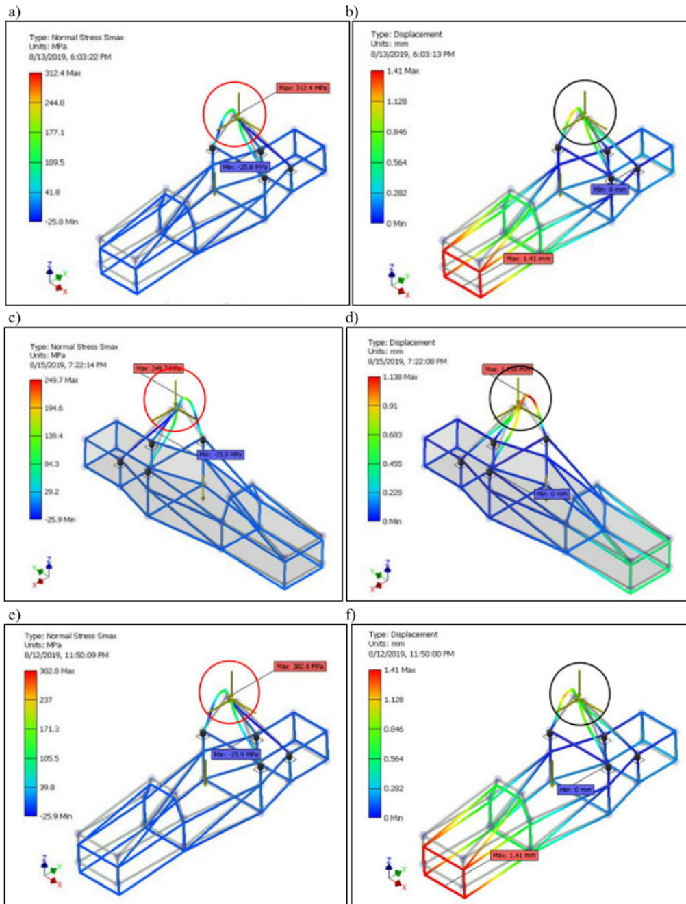
Fig. 6. Autodesk Inventor simulation results on normal stress and deflection: a) normal stress 502 mm, b) deflection 502 mm, c) normal stress 504 mm, d) deflection 504 mm, e) normal stress 506 mm, f) deflection 506 mm
