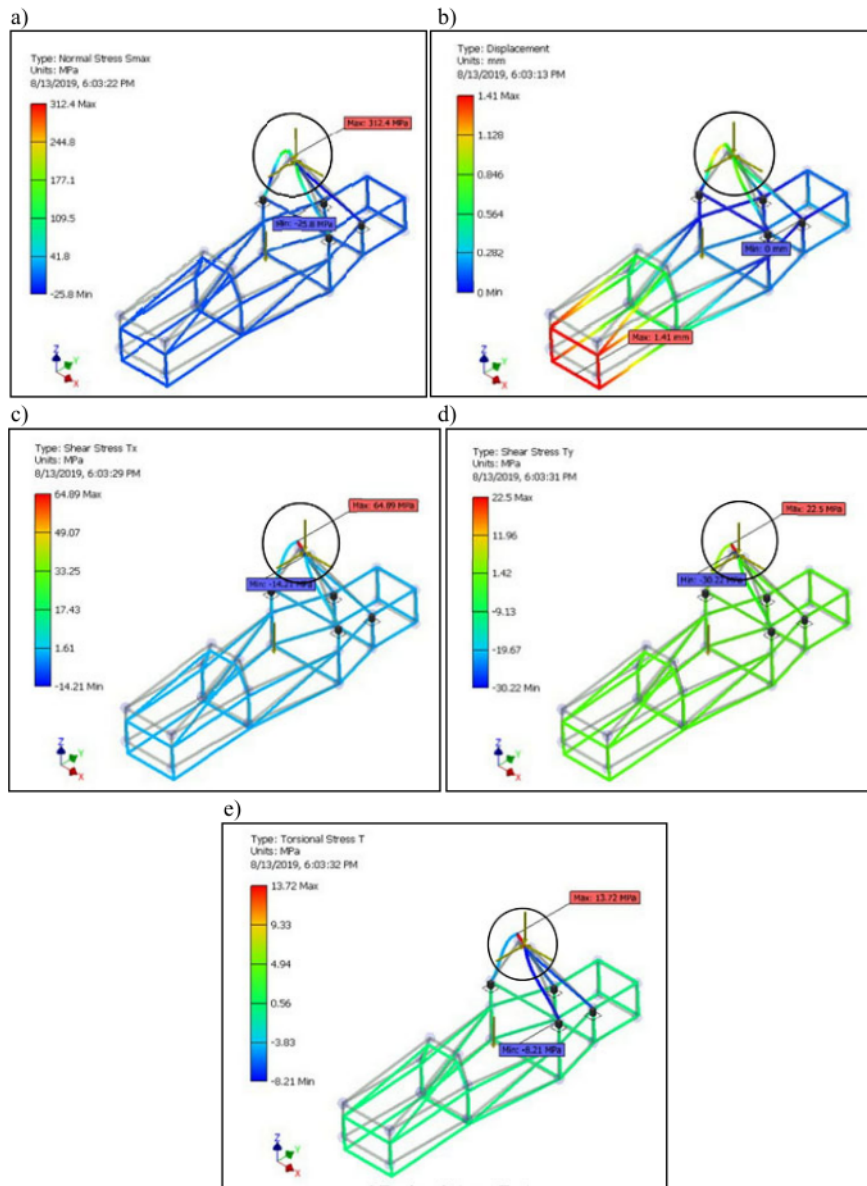
Fig. 4. Autodesk Inventor simulation results on chassis type A (roll-hoop height = 502 mm):a) normal stress test, b) deflection test, c) shear stress (T-x) test, d) shear stress (T-y) test, e) torsional stress test
