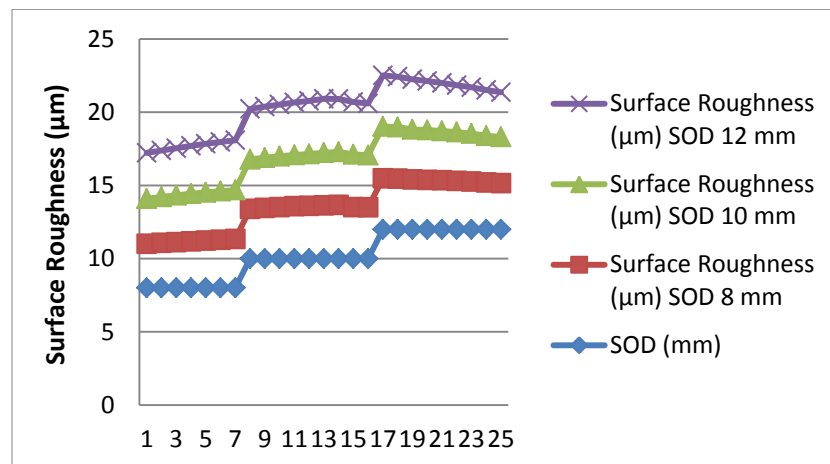
Figure 4. Surface roughness with coolant mineral water
