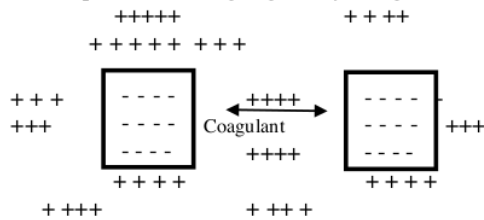
Figure 2. Attractive force of coagulant and colloid (flocs)
