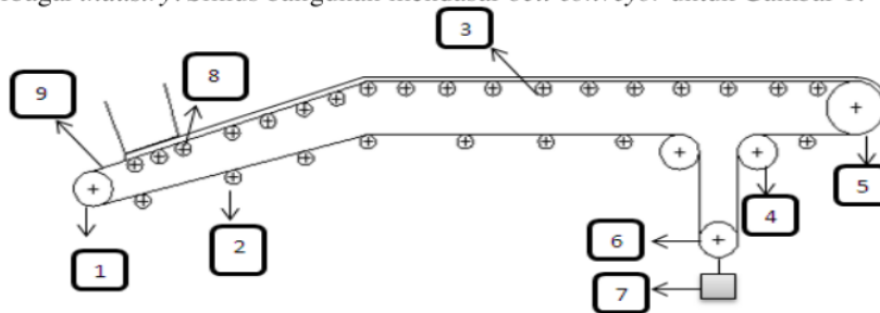
Gambar 1. Siklus Belt Conveyor
