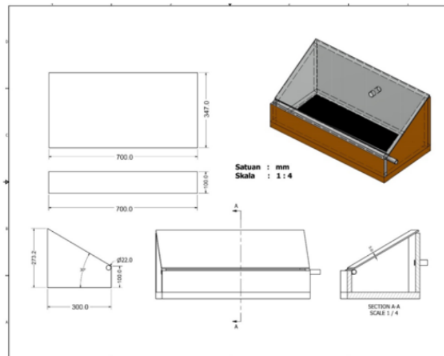
Gambar 5. Desain Alat Solar Distillation
