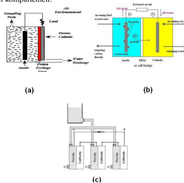
Gambar 1. Single Chamber (a), Double chamber (b), Stack (c)
