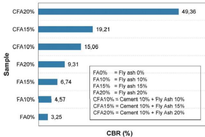
Figure 2. CBR test result
