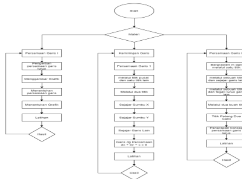
Gambar 3. Flowchart Materi
