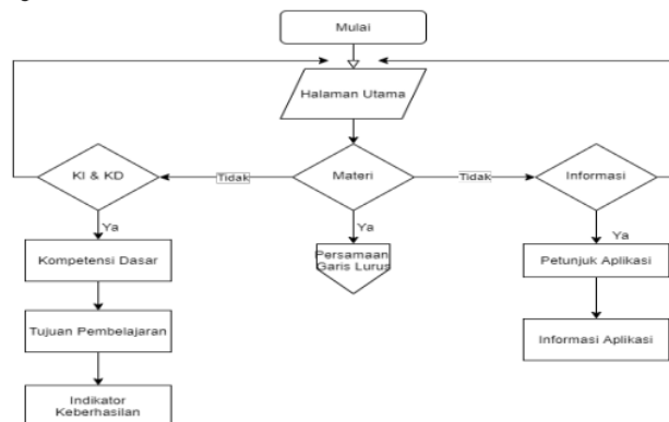
Gambar 2. Flowchart media
