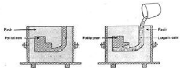
Gambar 1. Prinsip pengecoran evaporative
