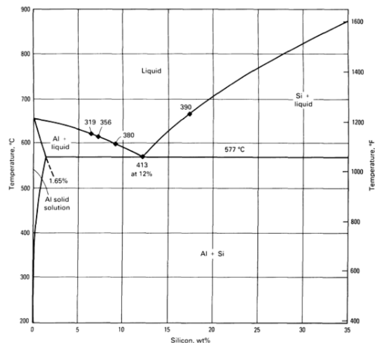
Gambar 2. Diagram fasa paduan Al-Si (ASM Handbook, 2004)
