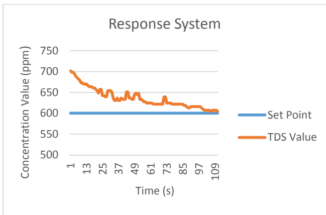
Fig. 12. Response system with initial value 700 ppm
