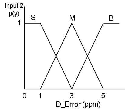
Fig. 7. Membership function of delta error
