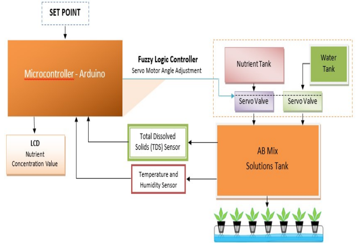
Fig. 2. Control system design for hydroponic concentration
