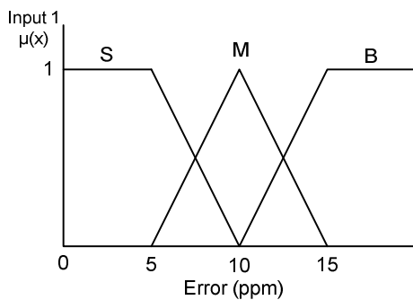
Fig. 6. Membership function of error
