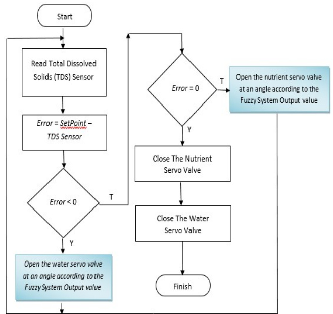
Fig. 3. Flowchart control process
