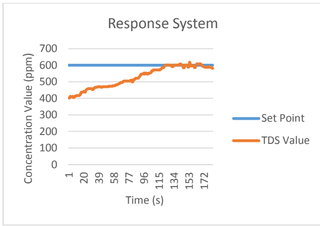
Fig. 11. Response system with initial value 400 ppm
