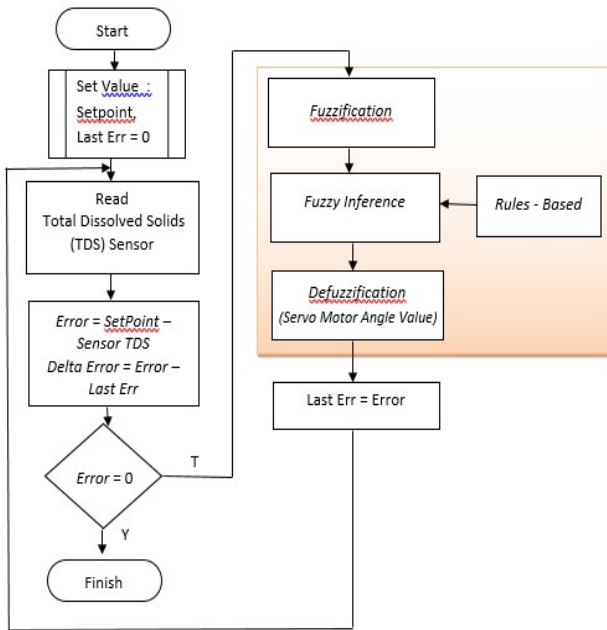
Fig. 4. Fuzzy inference system
