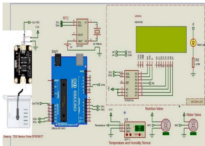
Fig. 9. Electronic Circuit
