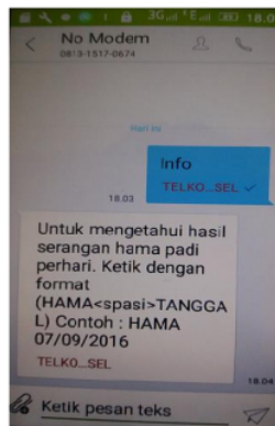
Gambar 4 Format SMS
