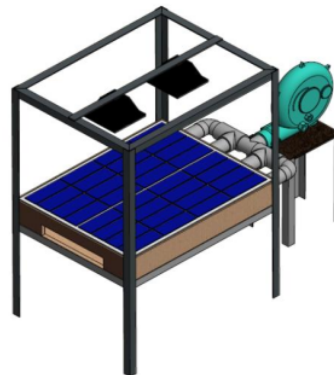
Gambar 3. Simulator Panel Surya
