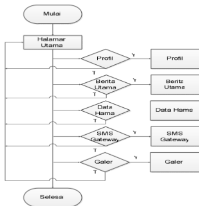
Gambar 1. Diagram Alir User Web
