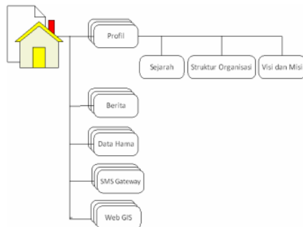
Gambar 5 Site Map Website BPTPH
