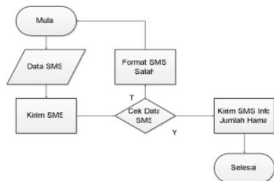
Gambar 2 Flowchart User SMS Gateway
