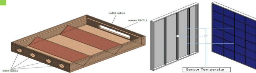
Gambar 4. Instalasi Penelitian
