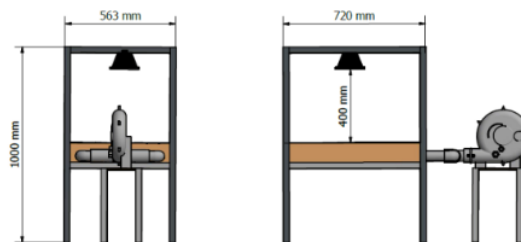
Gambar 1. Solar Simulator
