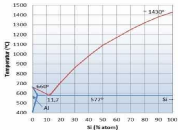
Gambar 6. Diagram Fasa Al-Si
