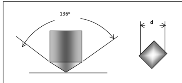
Gambar 7. Indentor Vickers
