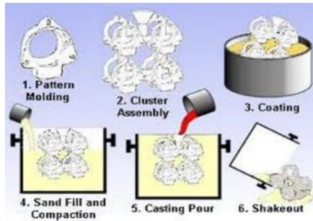
Gambar 2. Pengecoran Evaporative
