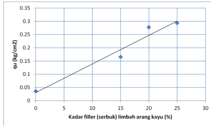
Gambar 3.6 Hubungan Nilai q_u vs prosentase arang
