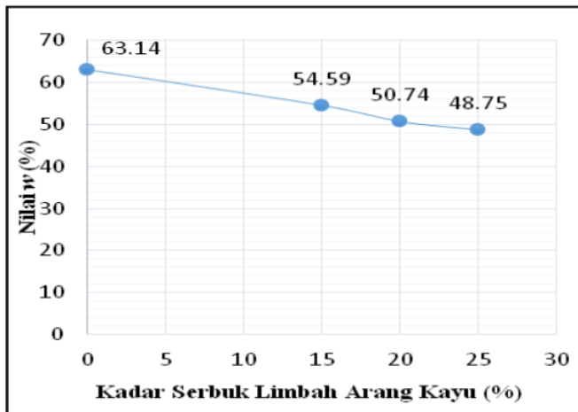
Gambar 3.2 Hubungan Nilai w vs prosentase arang
