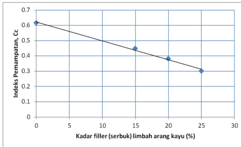
Gambar 3.5 Hubungan Nilai Cc vs prosentase arang
